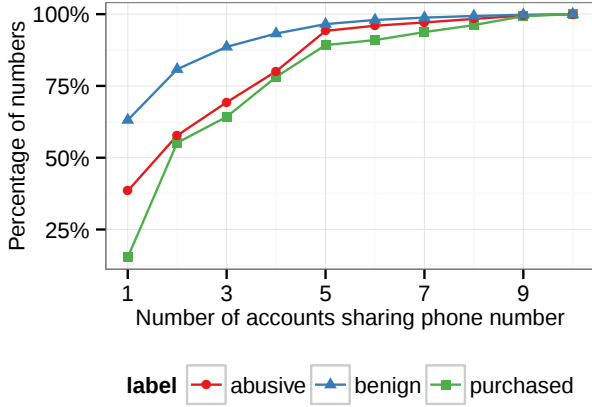
Figure 4: CDF of the size of account clusters all verified with the same phone number.
