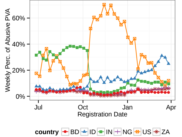
Figure 2: Weekly breakdown of the top 6 country codes associated with abused phone numbers. The most popular origins of numbers are the United States (US), India (IN), Indonesia (ID), Nigeria (NG), South Africa (ZA), and Bangladesh (BD).
