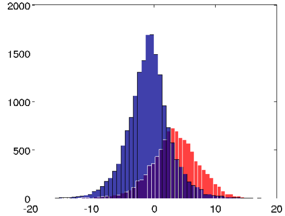
Figure 15. Histograms for the best cat neuron on the test set. Red: the histogram for cat images. Blue: the histogram for random distractors.
