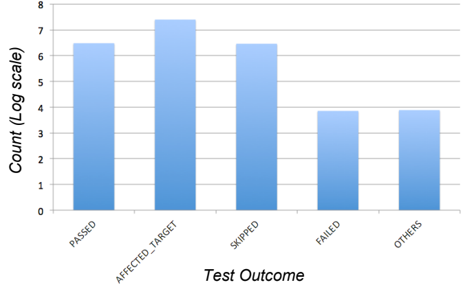
Fig. 4. Distribution of Overall Test Outcomes.
