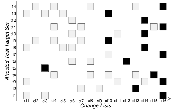
Fig. 2. Changelists and associated test targets.
