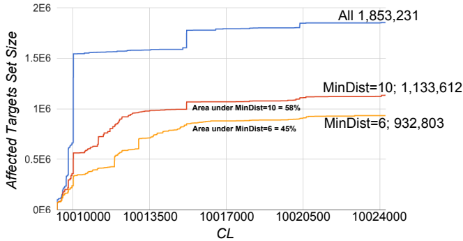
Fig. 12. Simulating with \text{MinDist} = 6 and 10.
